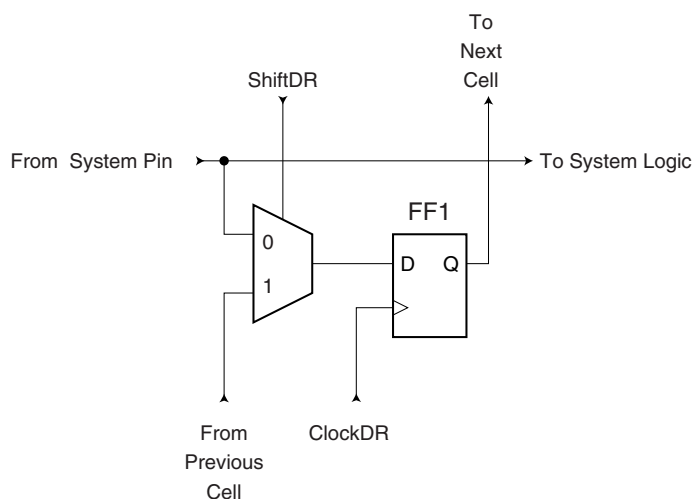
Figure 23-5. Observe-only Cell
