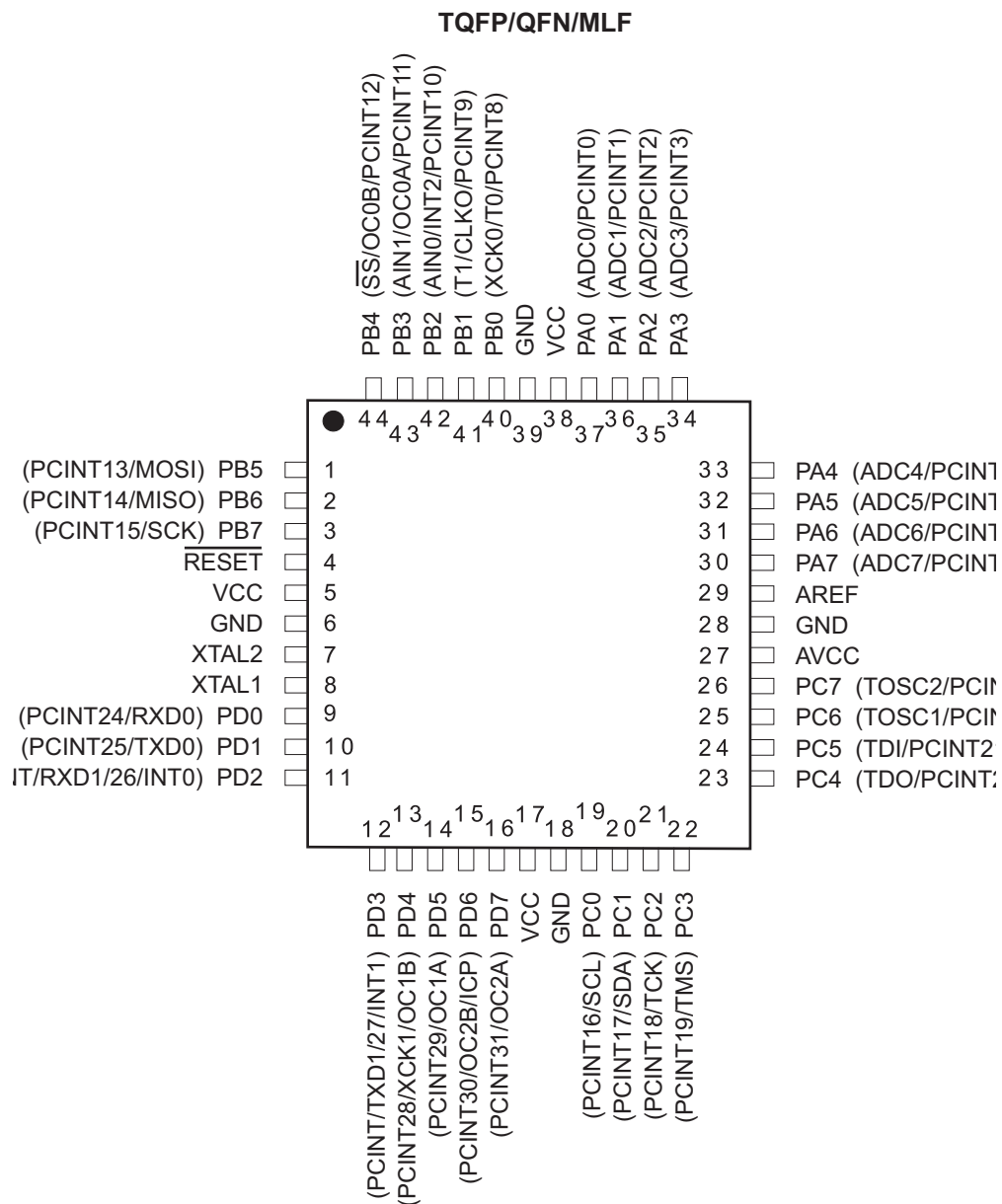
Figure 1-1. Pinout ATmega164P/324P/644P
