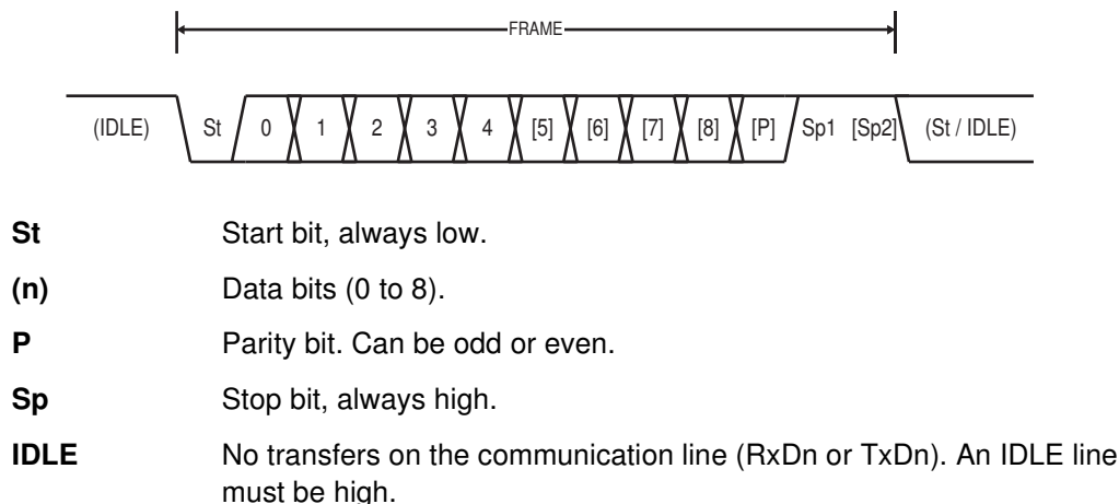
Figure 17-4. Frame Formats
