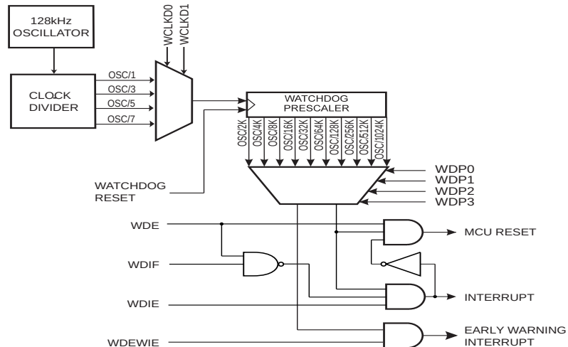
Figure 9-8. Watchdog Timer
