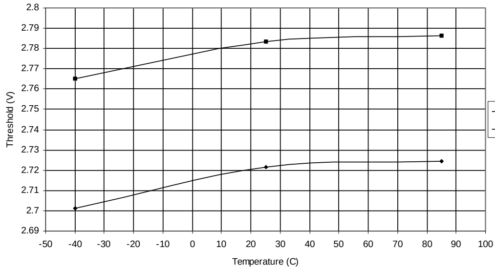
Figure 27-25. BOD Voltage (2.9V level) vs. Temperature
