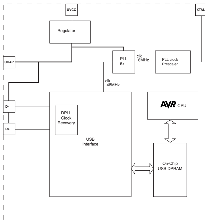
Figure 19-1. USB controller Block Diagram overview
