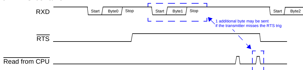
Figure 17-9. \overline{\text{RTS}} behavior
