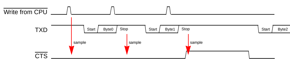
Figure 17-10. \overline{\text{CTS}} behavior
